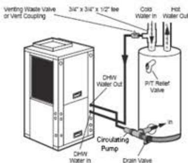
Figure 2: Typical Desuperheater Installation
