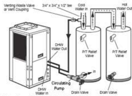
Figure 3: Desuperheater Installation In Preheat Tank
